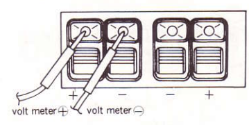
Fig. 2-4 SPEAKER TERMINAL
