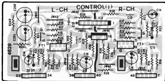
3-4. F-4629 Control Amp. Circuit Board (Stock No. 00826001) Component Side
