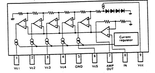
•BA6137(L.E.D Drive)
