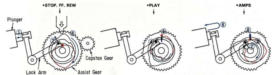
2-4. Cam Positions in the Modes of PLAY, FF, REW & STOP
