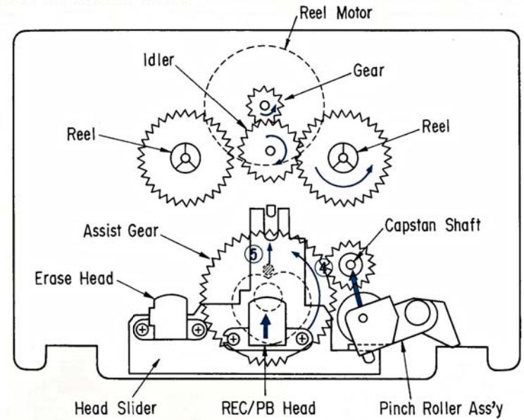
2-3. Front View of Mechanism Chassis
