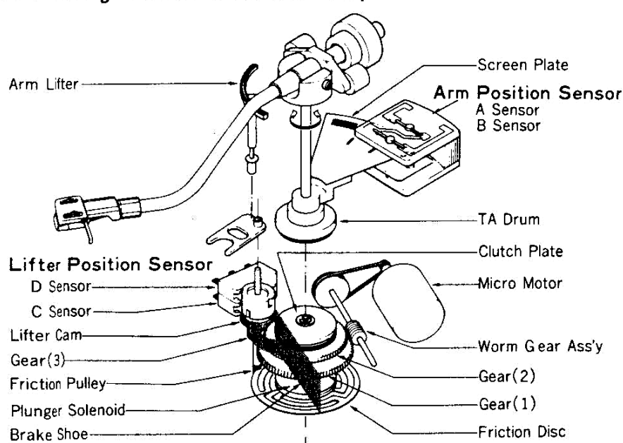
Fig. 2-1 Configuration of Mechanism Ass'y
