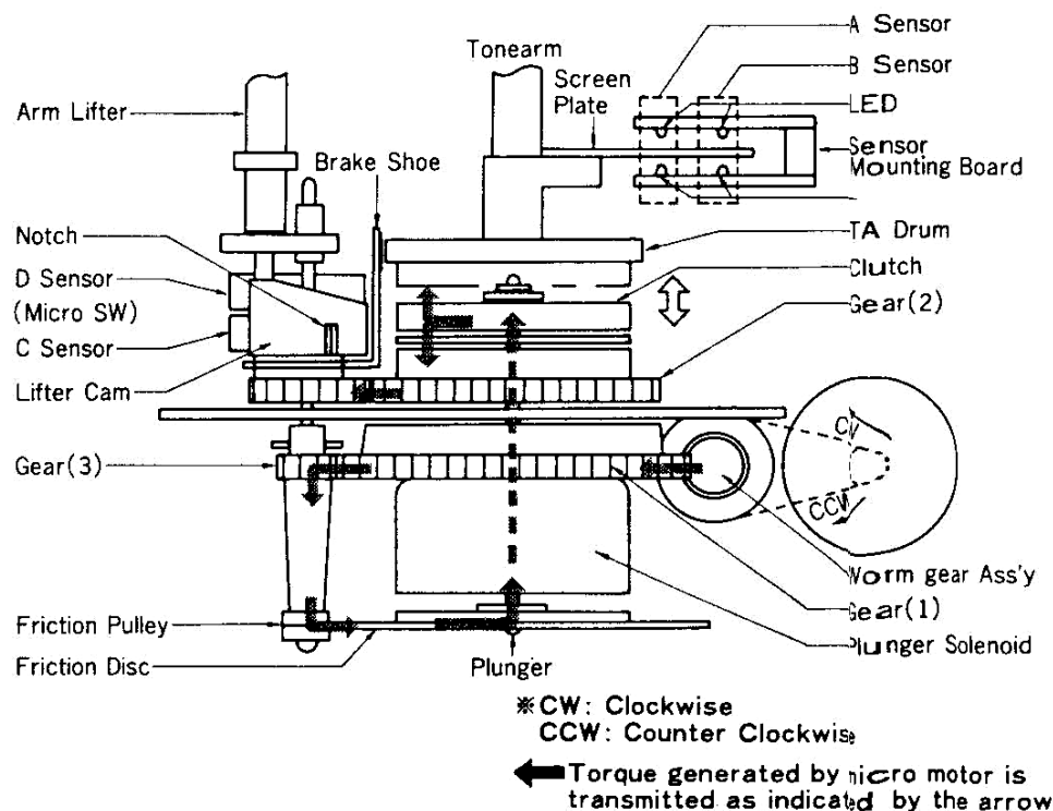
Fig. 2-2 Side View of Mechanism Ass'y and Movement of Gear Train
