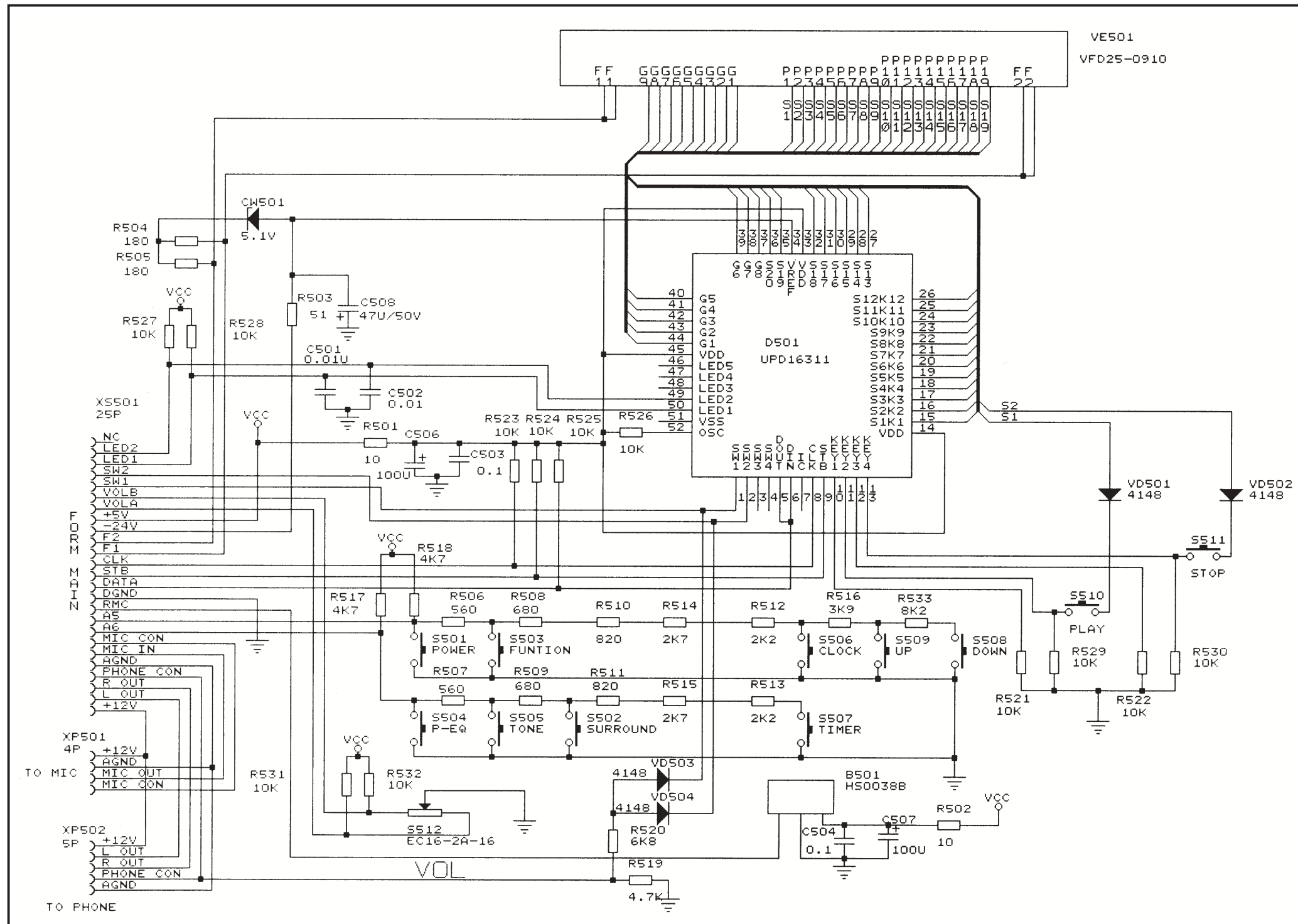
A750 KEY CIRCUIT
