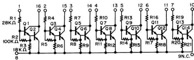
● BA-6250 (7 Transistor Array)
