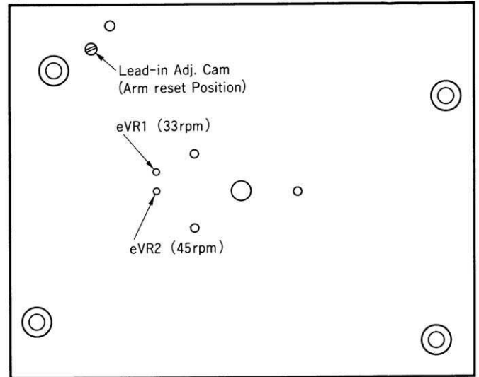
Fig.3-2 Bottom View
