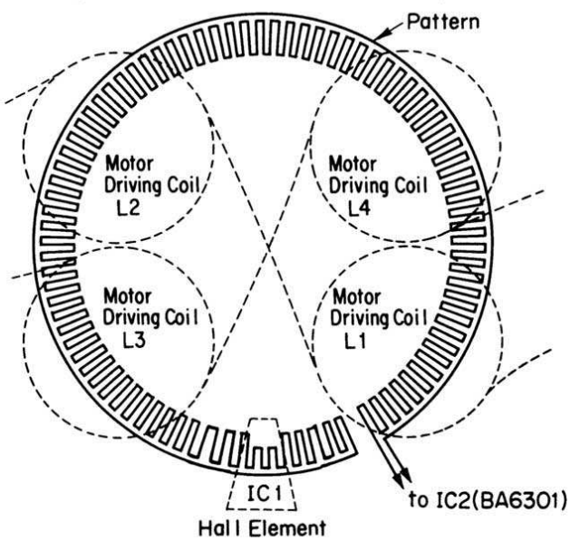
Pattern drawing of motor section (F-4892 Motor Control Circuit Board)
