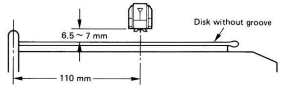
Fig.3-5 (b)
