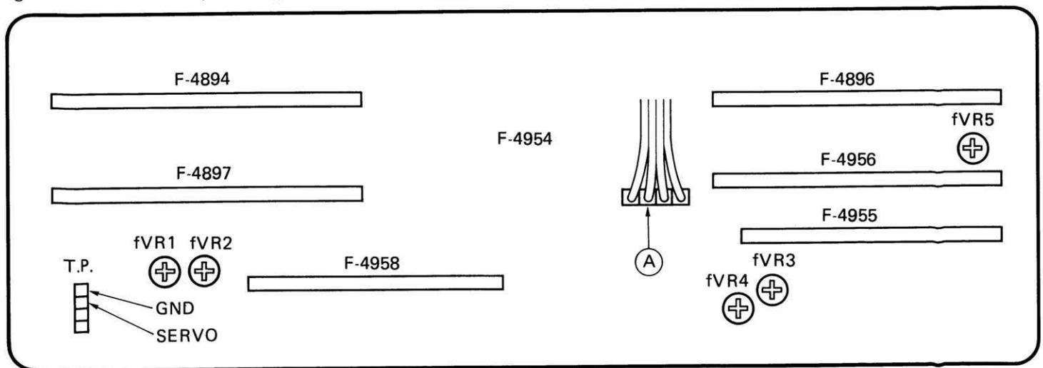
Fig.3-4 F-4954 Test & Adjustment points
