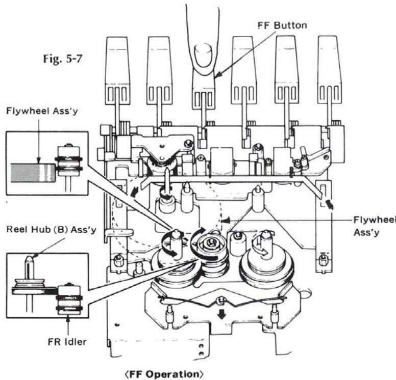
<FF Operation>
