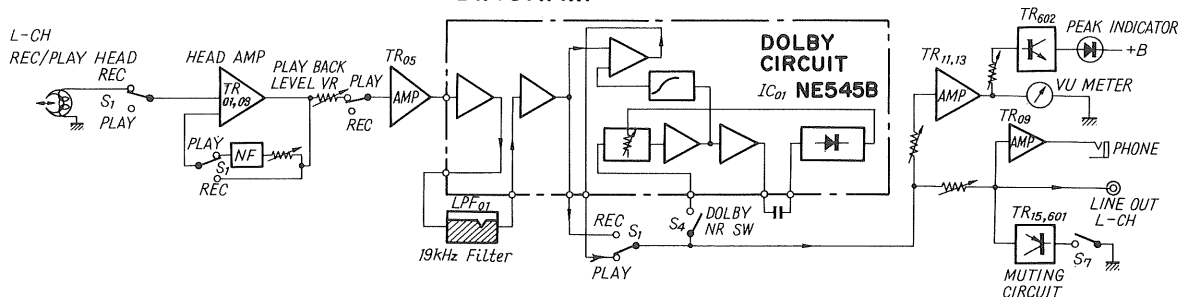
PLAYBACK OPERATION BLOCK DIAGRAM
