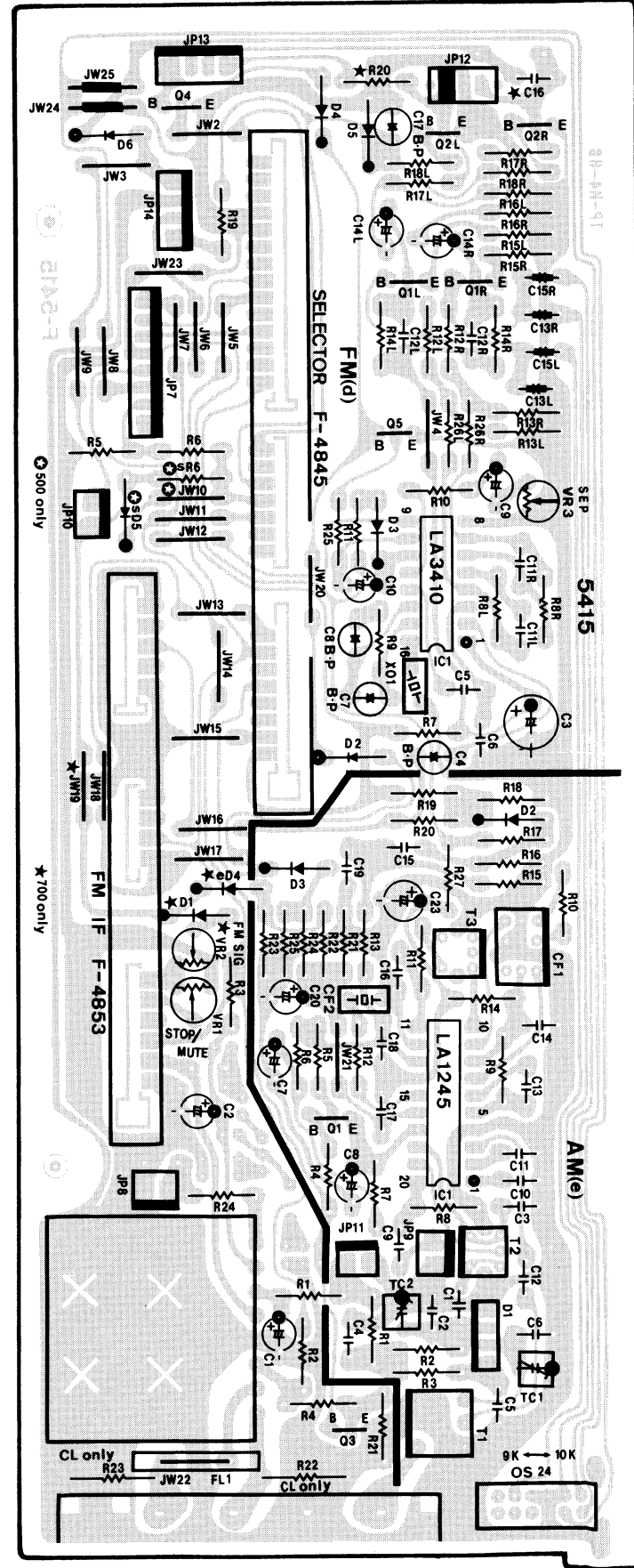
3-12. F-5415 Tuner Board Component Side
