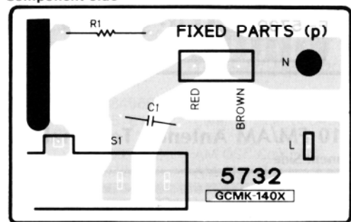
5-4. F-5732 Power Switch Board Component Side
