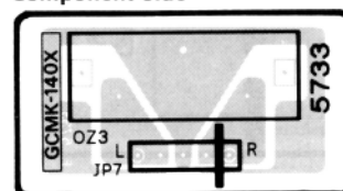
5-5. F-5733 OUTPUT Terminal Board Component Side
