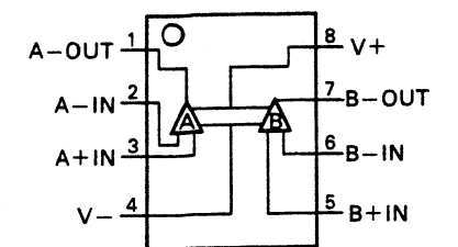
• NJM4558D/NJM2043D-D (Operational Amp. IC)
