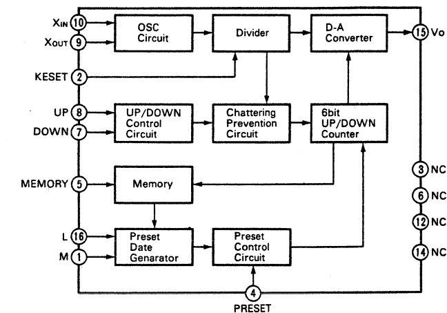
• M50601P (D-A Converter IC)
