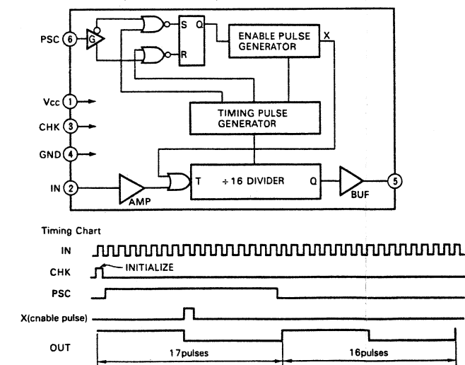
• \mu PB553AC (Prescaler IC)
