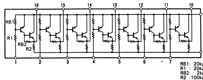
• \mu PA80C (FL Display Drive IC)
