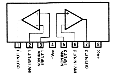
• M5220L (Audio Pre Amp. IC)
