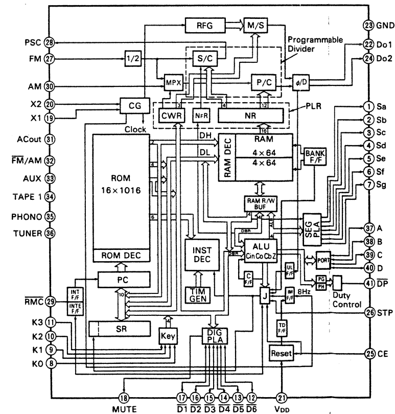
• \mu PD1704C-011 (FM/AM PLL Synthesizer & Control IC)
