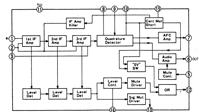
• HA12412 (FM Detector IC)
