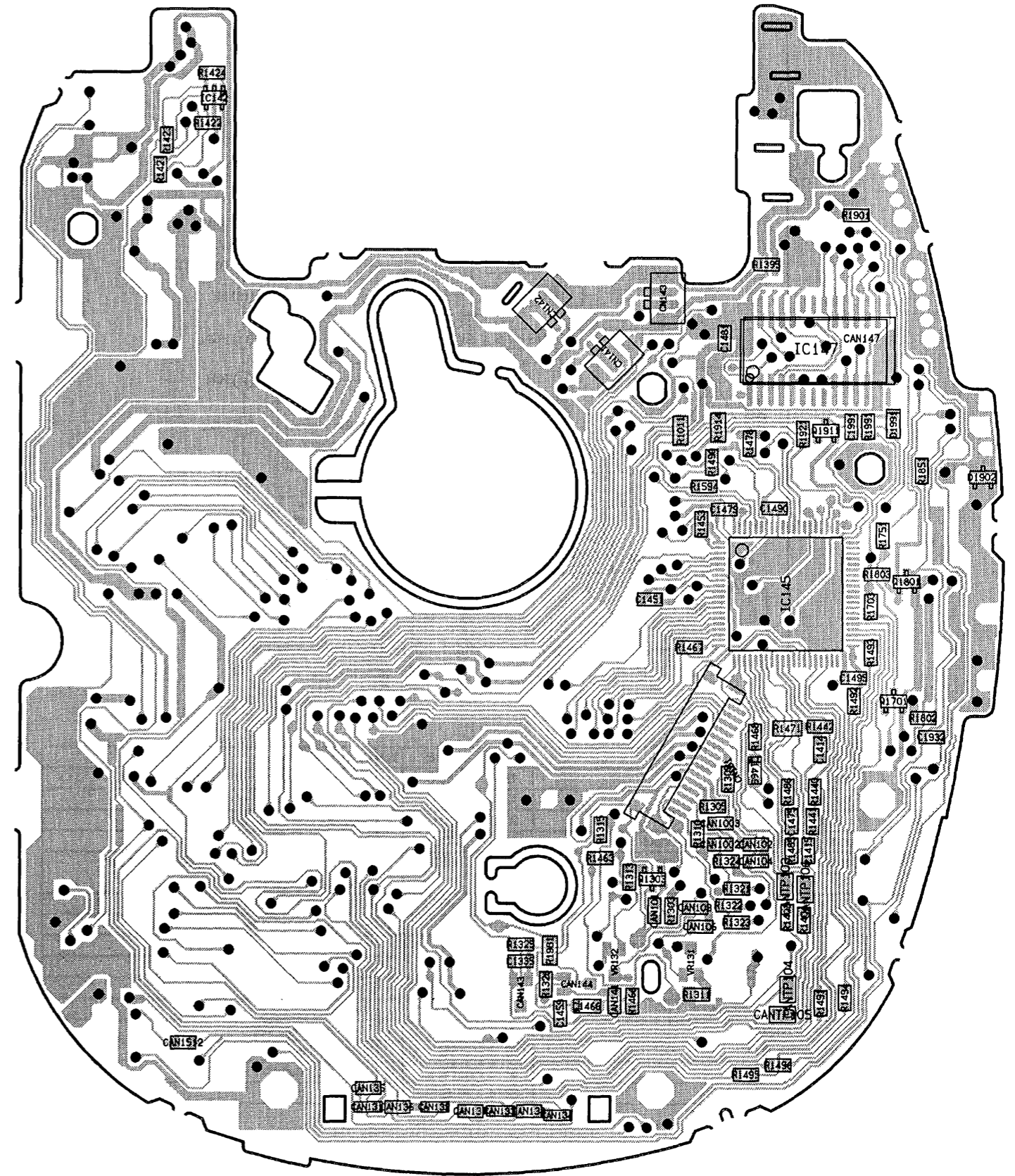
TOP VIEW
