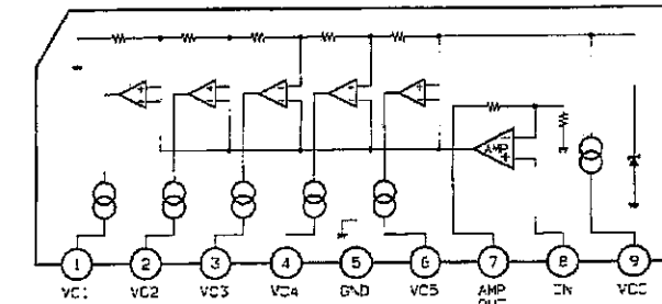
IC902 LB1433N (LED Level Meter Driver)
