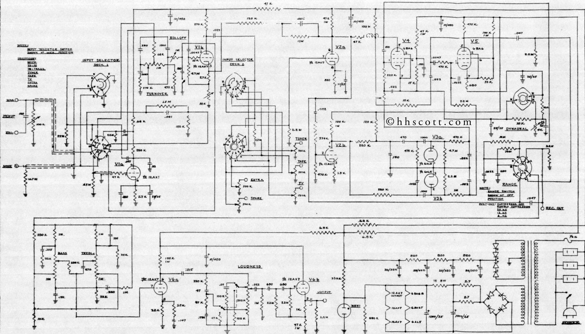
121 DYNABAL EQUALIZER PREAMPLIFIER CIRCUIT DIAGRAM
