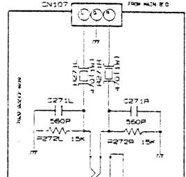
PCB2-4 (HEAD PHONE)
