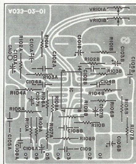
MIC PREAMP BOARD
