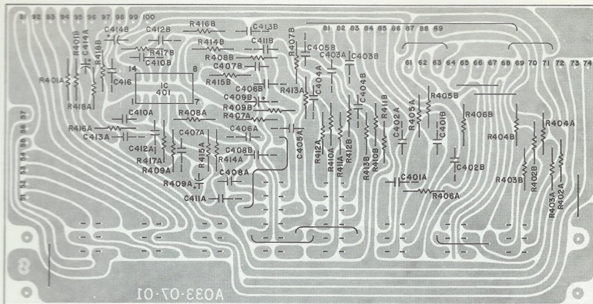
FUNCTION SWITCH and FILTER BOARD A033-07-01
