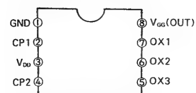
MN3101:IC108
