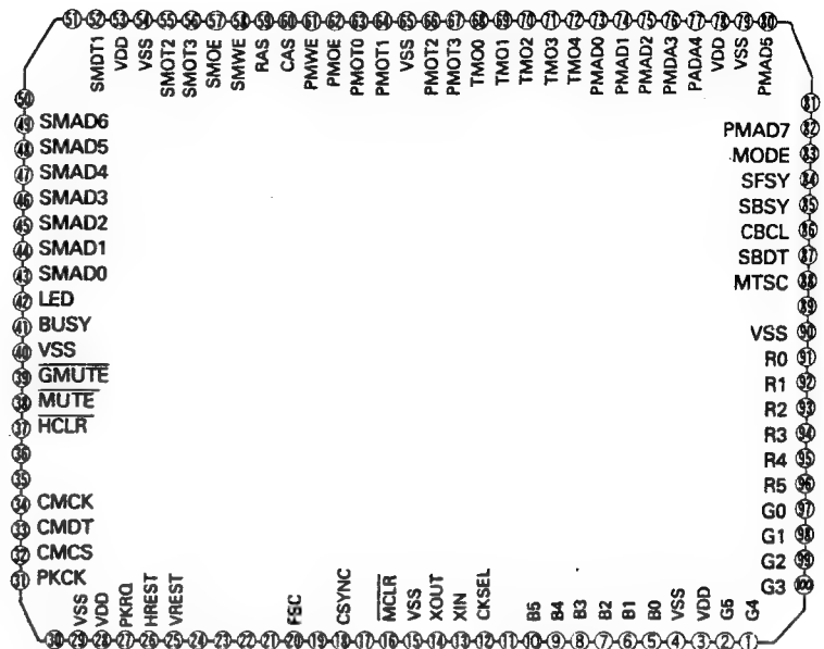
IC404 : KA2195D
