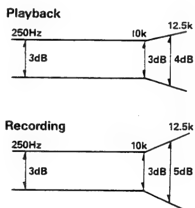
Fig. 1 Allowable Playback/Recording Frequency Response Zone
