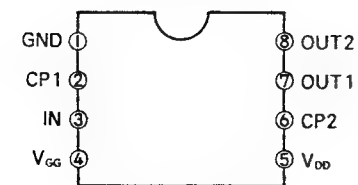
MN 3007:IC107
