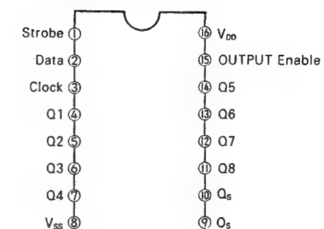
MC14094:IC303
