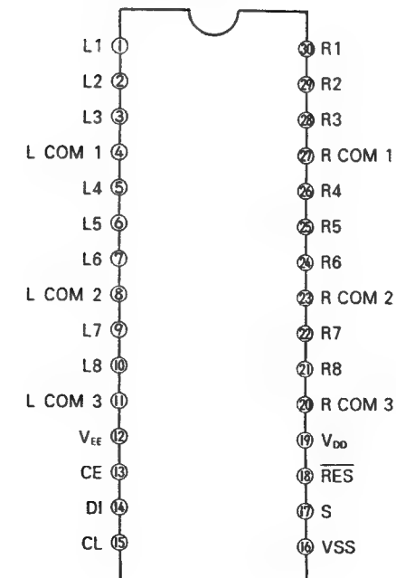
LC 7822:IC402
