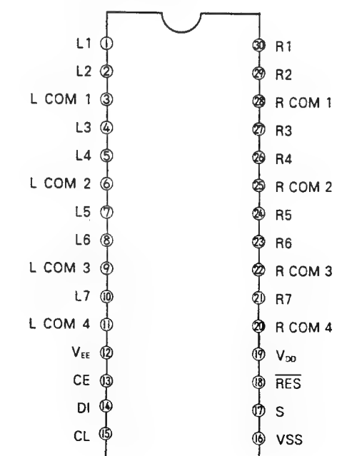
LC7823:IC404
