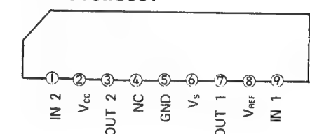
TA7291S:IC501
