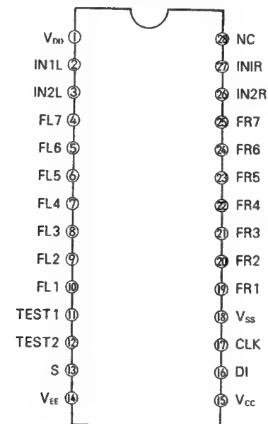
NJU 73052:IC103
