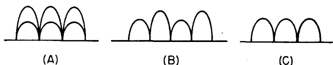
BALANCE WAVEFORMS FIGURE 2
