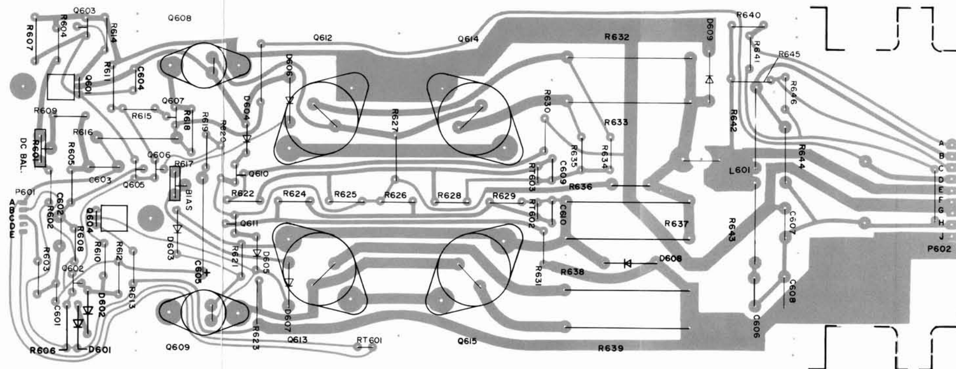
POWER AMPLIFIER BOARD A6 COMPONENT SIDE FIGURE 30
