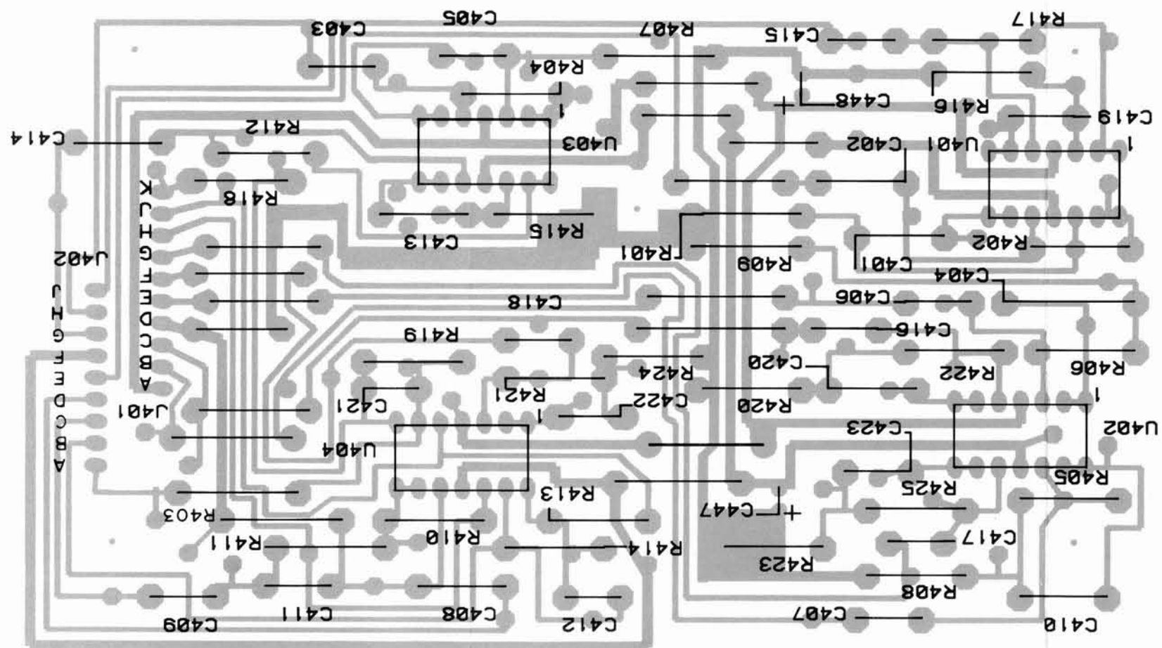
EQUALIZER BOARD A4 COMPONENT SIDE FIGURE 25
