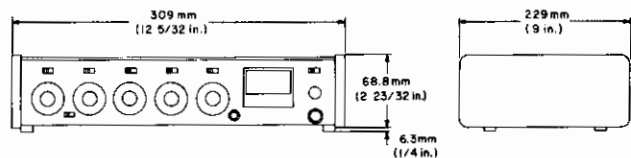
OVERALL DIMENSIONS FIGURE 1
