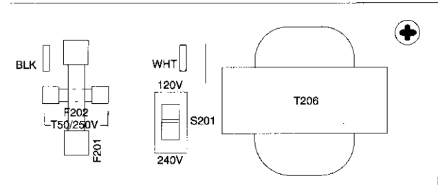
240 V WIRING FIGURE 3
