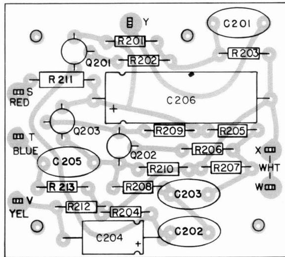
FIGURE 19. FILTER CIRCUIT BOARD PARTS LOCATION DIAGRAM
