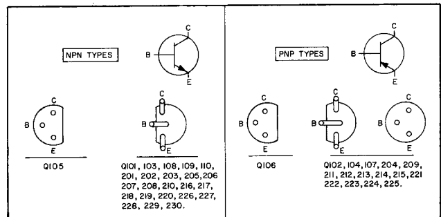
FIGURE 8. TRANSISTOR LEAD CODES
