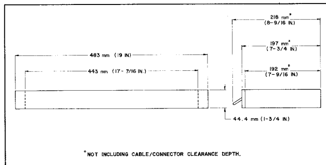
FIGURE 3. OVERALL DIMENSIONS
