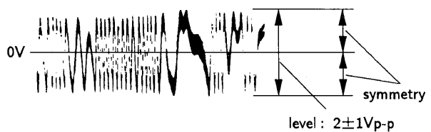
Traverse waveform
