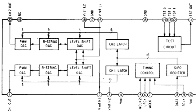
IC10 CXD1161P-3
