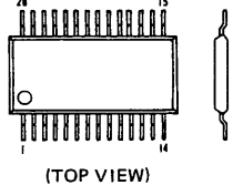
CXD2561BM
