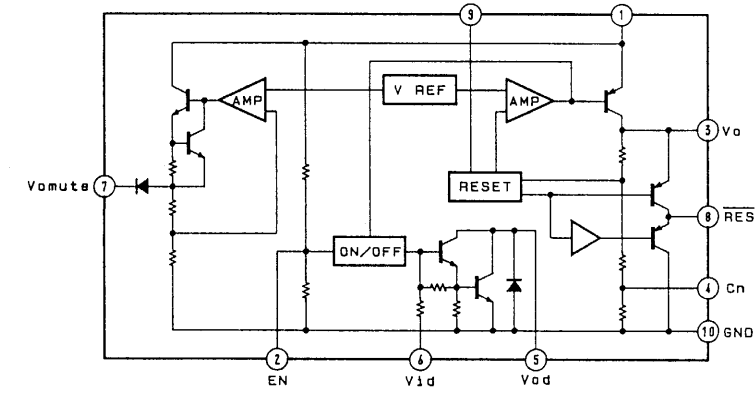
IC307 CXD8567AM
