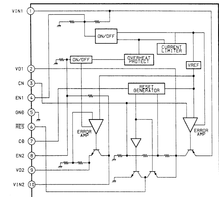
IC302 LA5601
