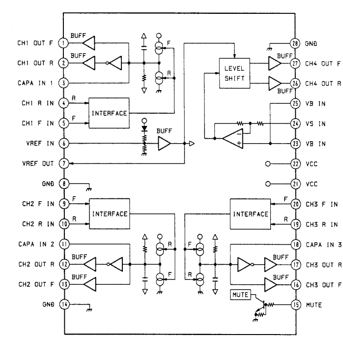
IC102 BA6392FP
