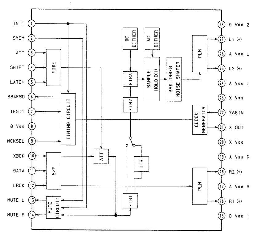
IC307 CXD8567AM
