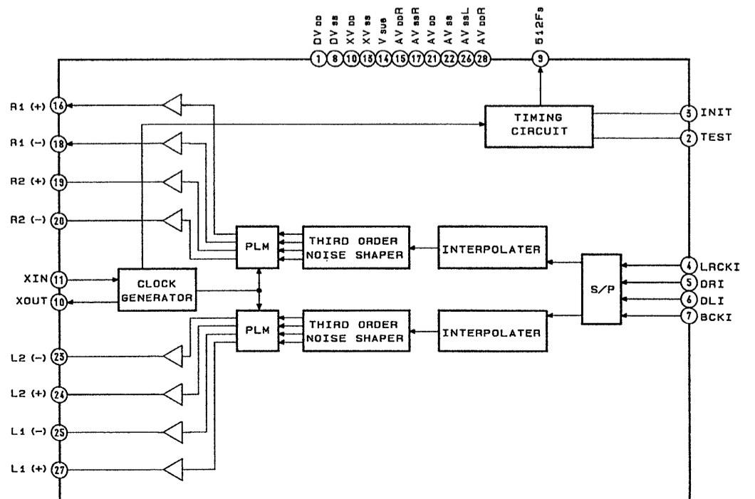
IC303 CXD2561AM
