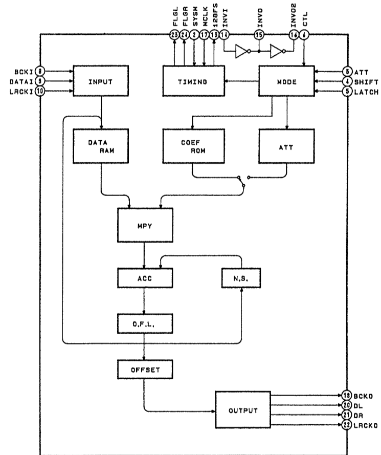
IC302 CXD2560M
