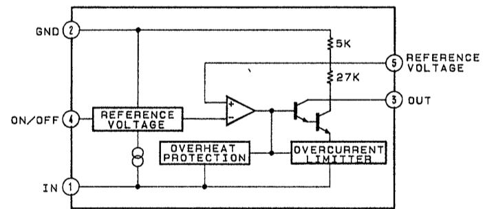
IC201 M5293L
