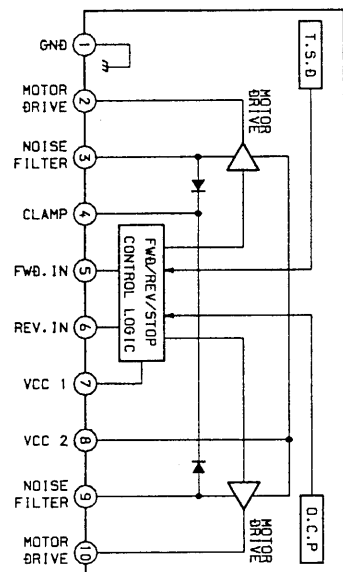
IC401 LB1641
