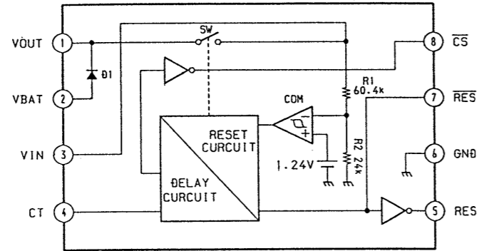
IC612 M62021FP-600C
