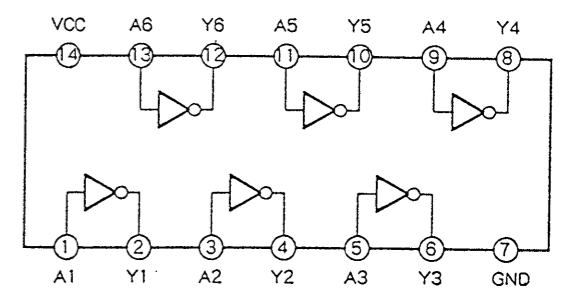
IC905 SN74HC04ANS-E20
