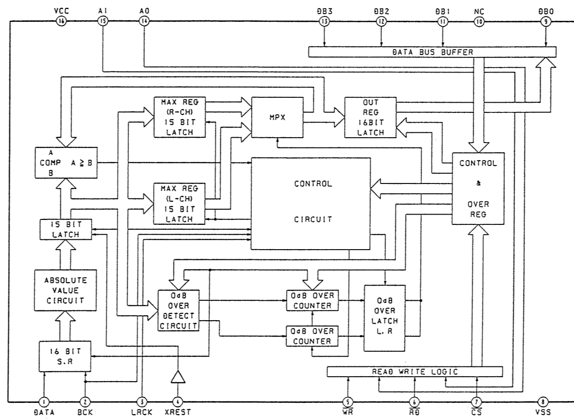
IC605 MSM6338RS
