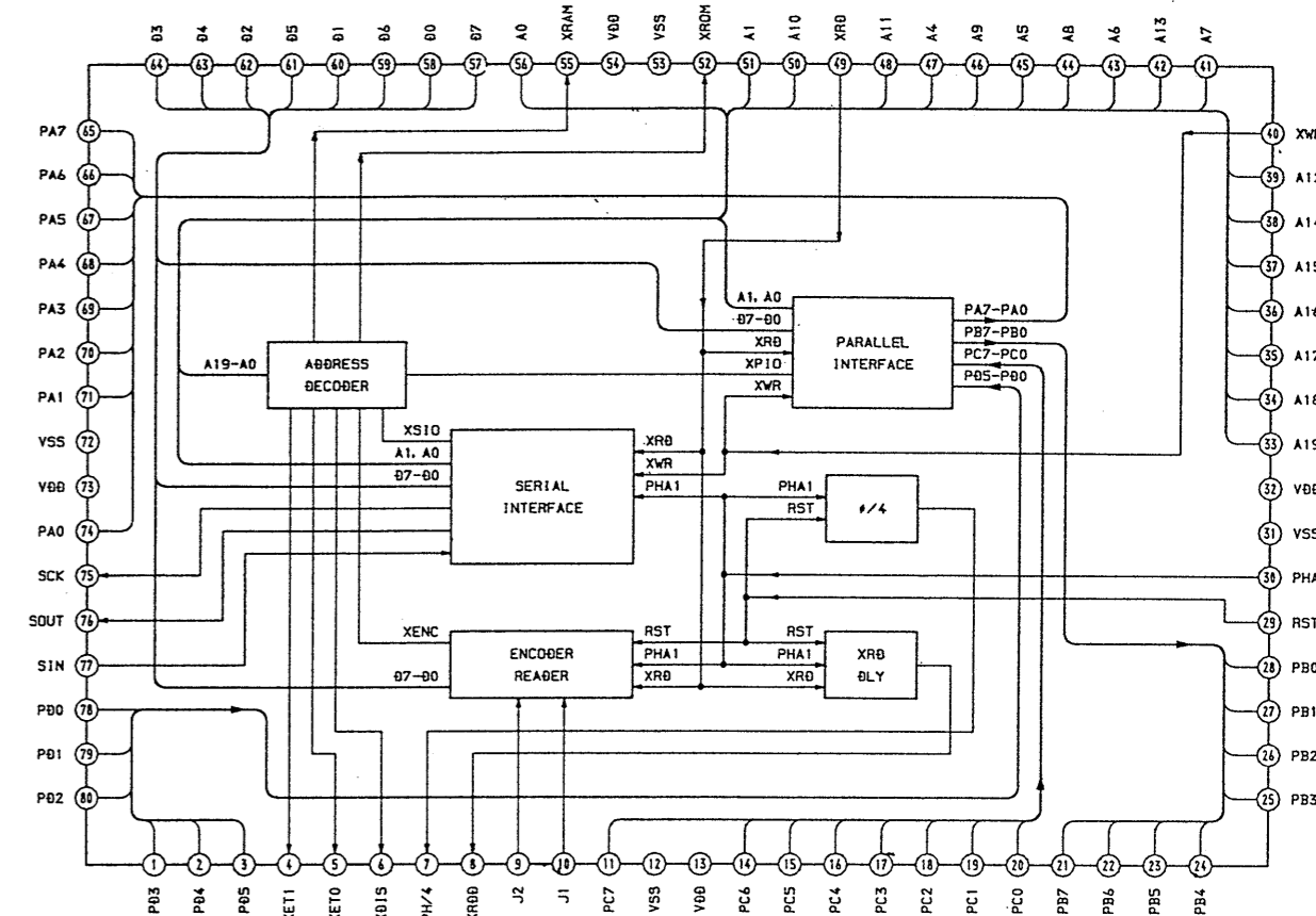
IC606 CXD8481Q
