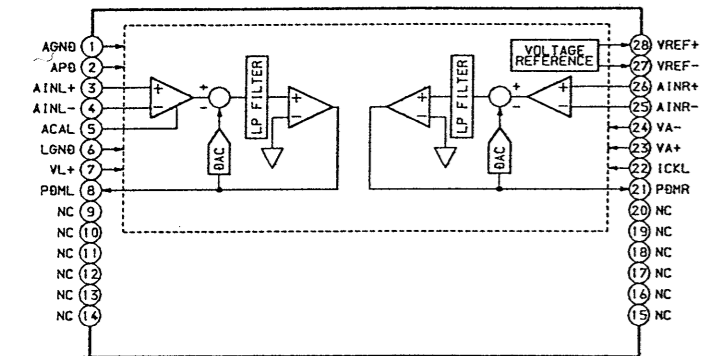
IC304 CXD8493M-E1
