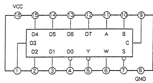
IC615 SN74HC151ANS-E20
