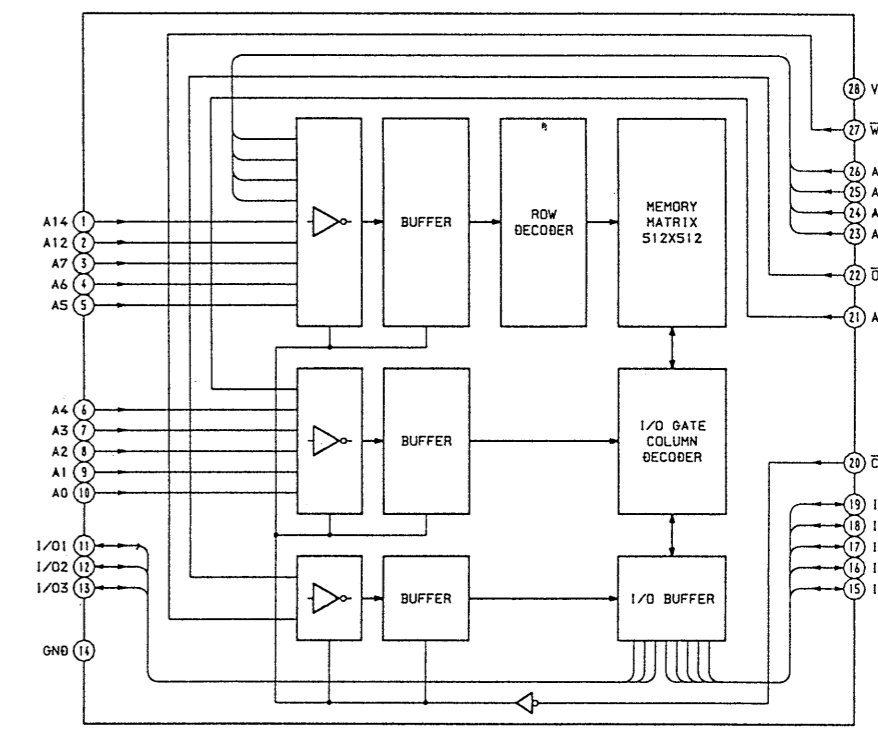
IC608, 609 CXK58257AM-10LL-T6
