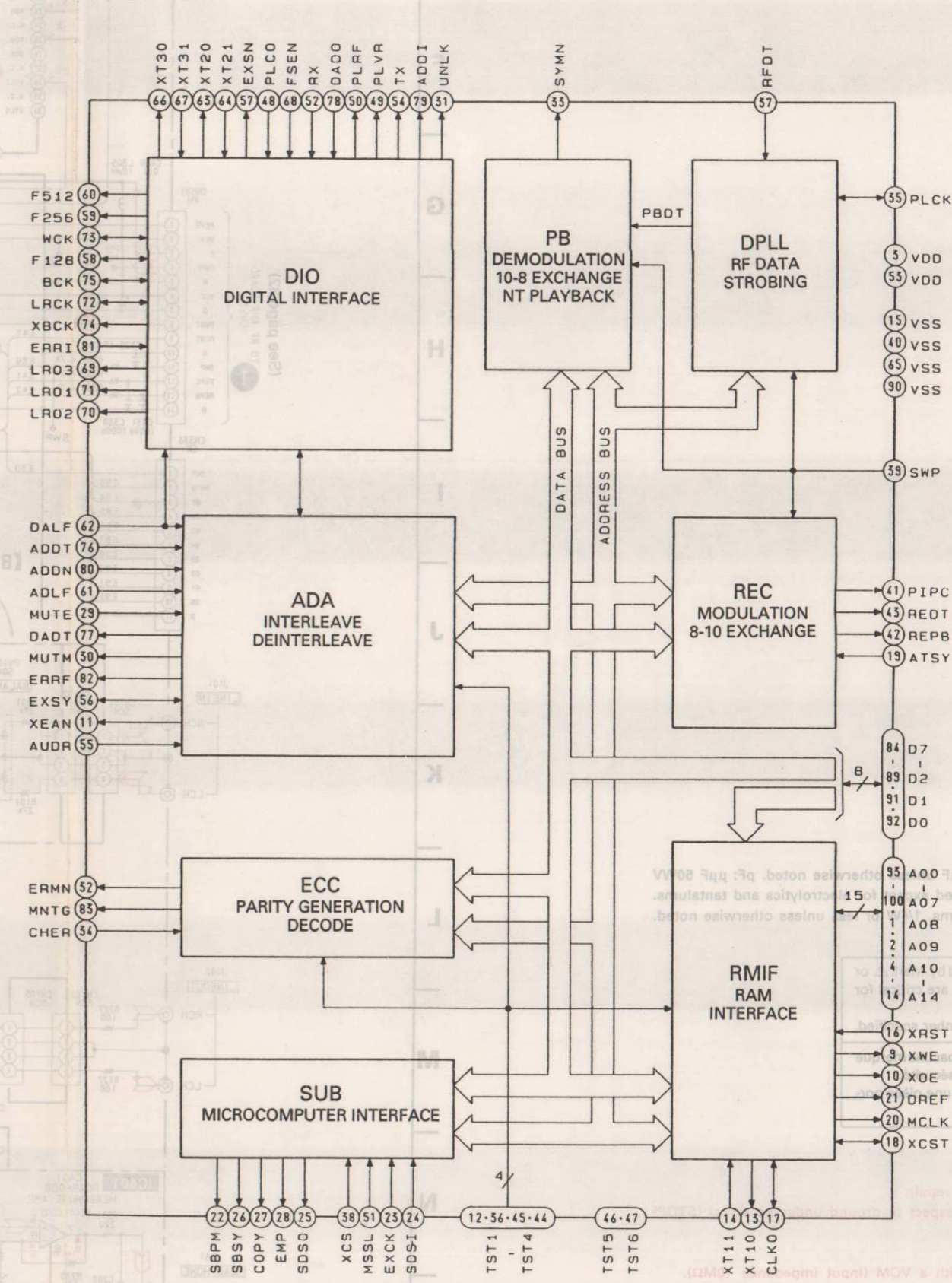
IC307 CXD2601AQ
