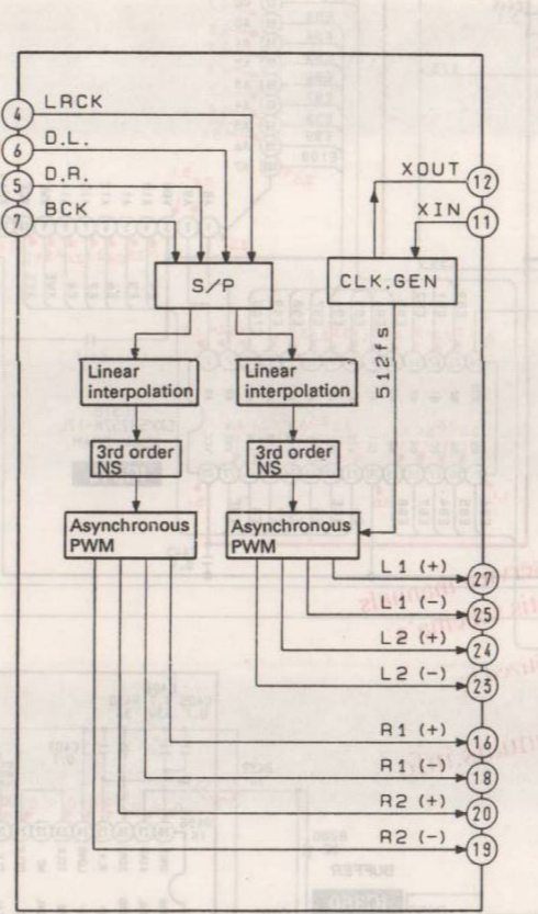
IC362 CXD2561M
