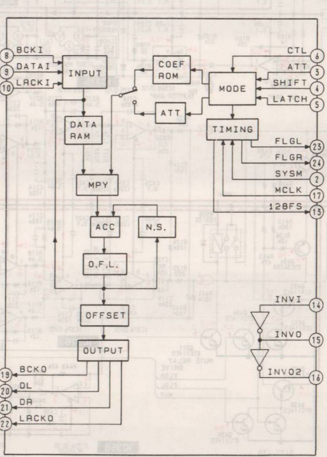
IC363 CXD2560M
