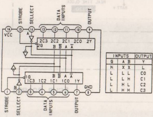
IC305 SN74HC153NS
