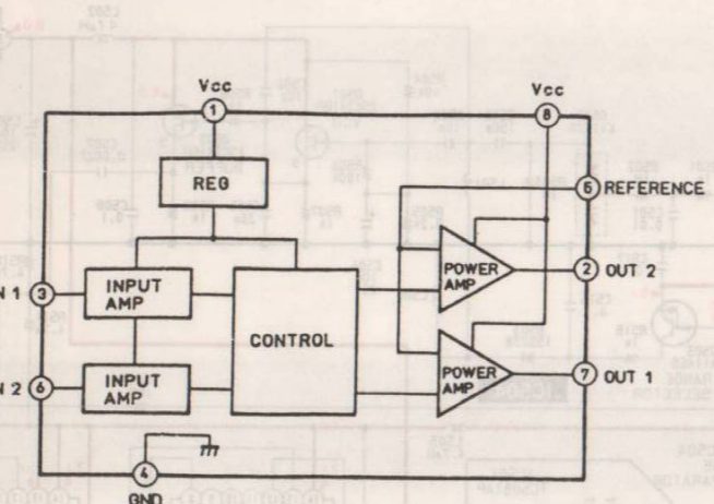
IC319,320 M54641L
