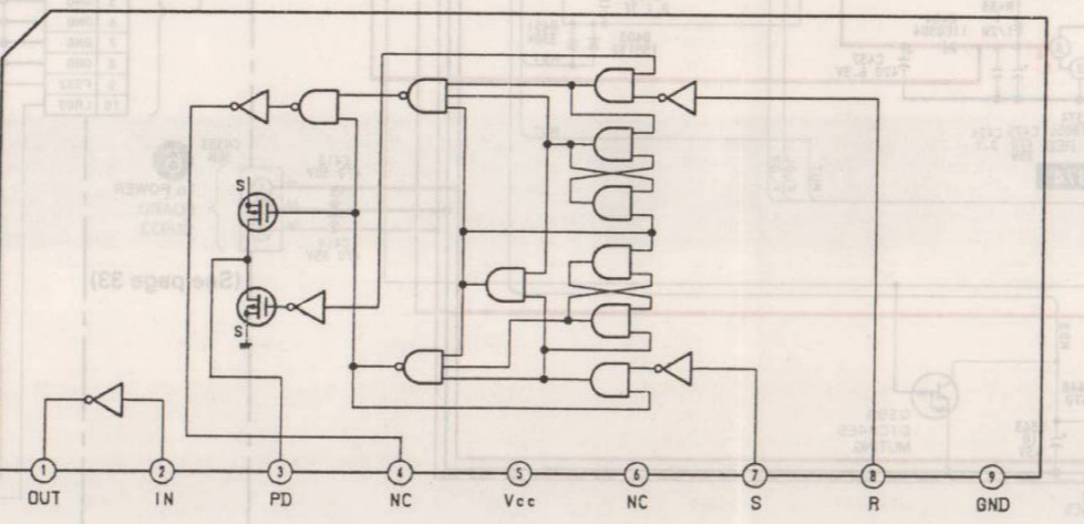
IC504 TC5081AP
