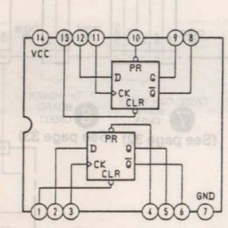
IC309 SN74HC74NS
