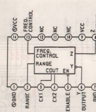
IC308 SN74LS624N
