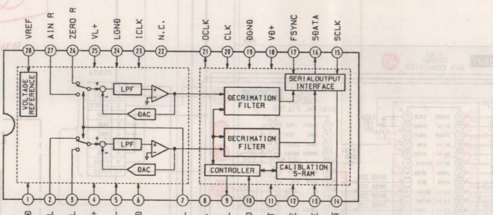
IC359 AK5339
