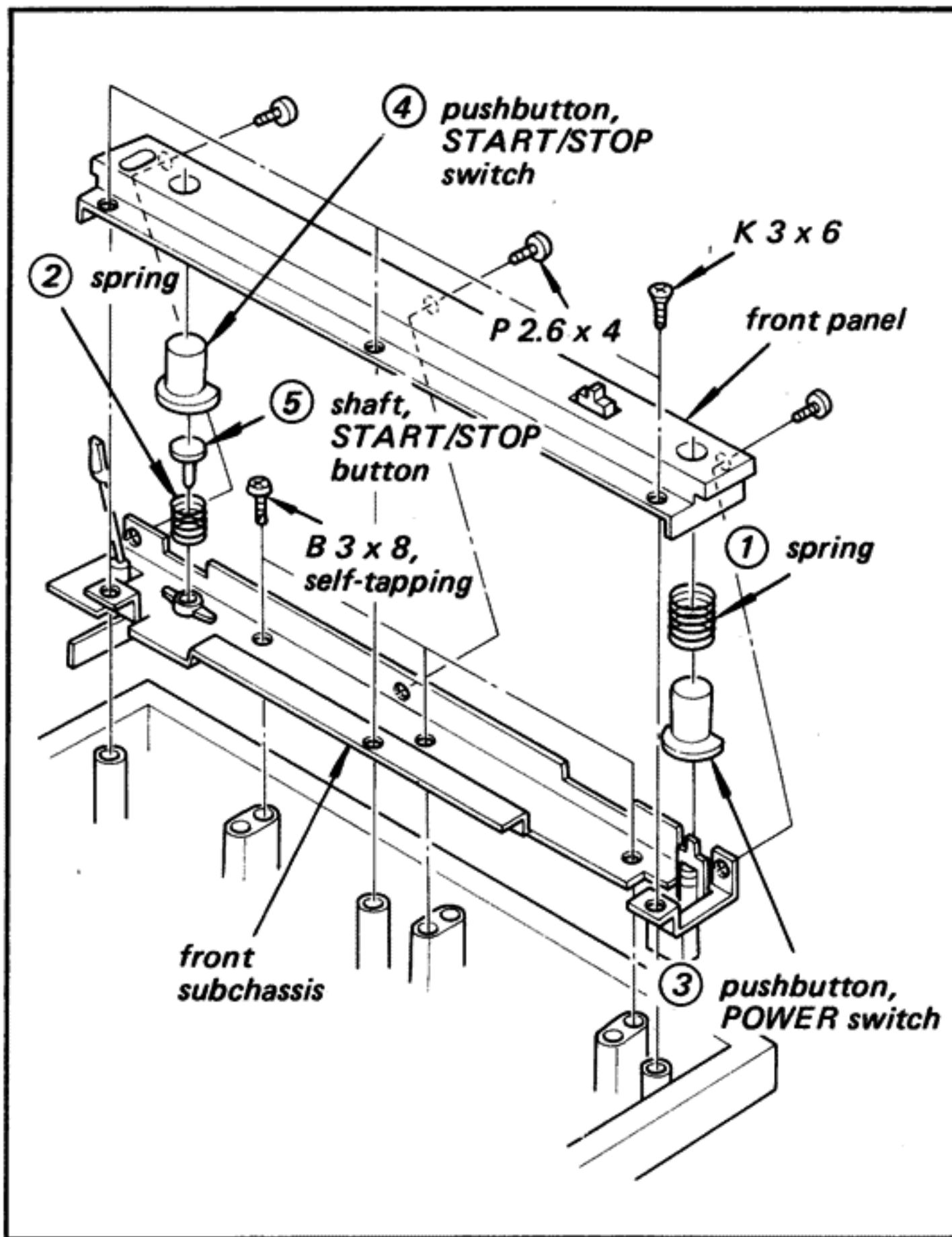
Fig. 2-12. Front panel/front subchassis removal
