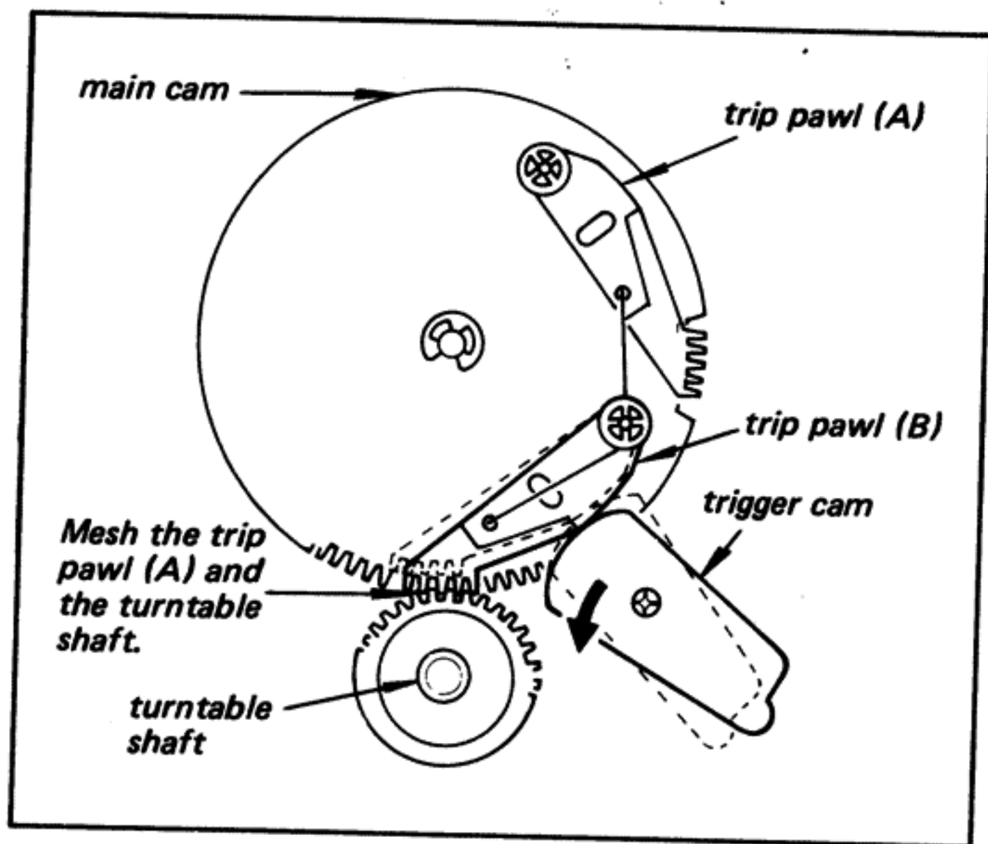
Fig. 3-16. Microswitch adjustment (3)
