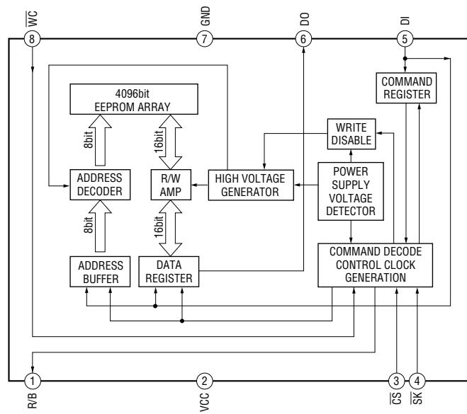
IC702 BR9040F-WF2
