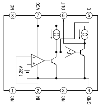
IC701 M51957BFP-600C
