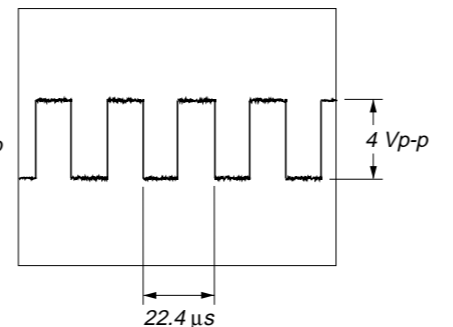
⑰ IC509 ⑤⑤ (LRCK) (CD Play)
