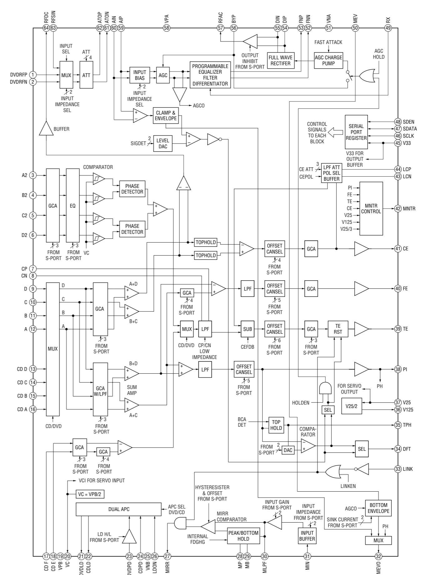
IC001 CXD1881AR-2
