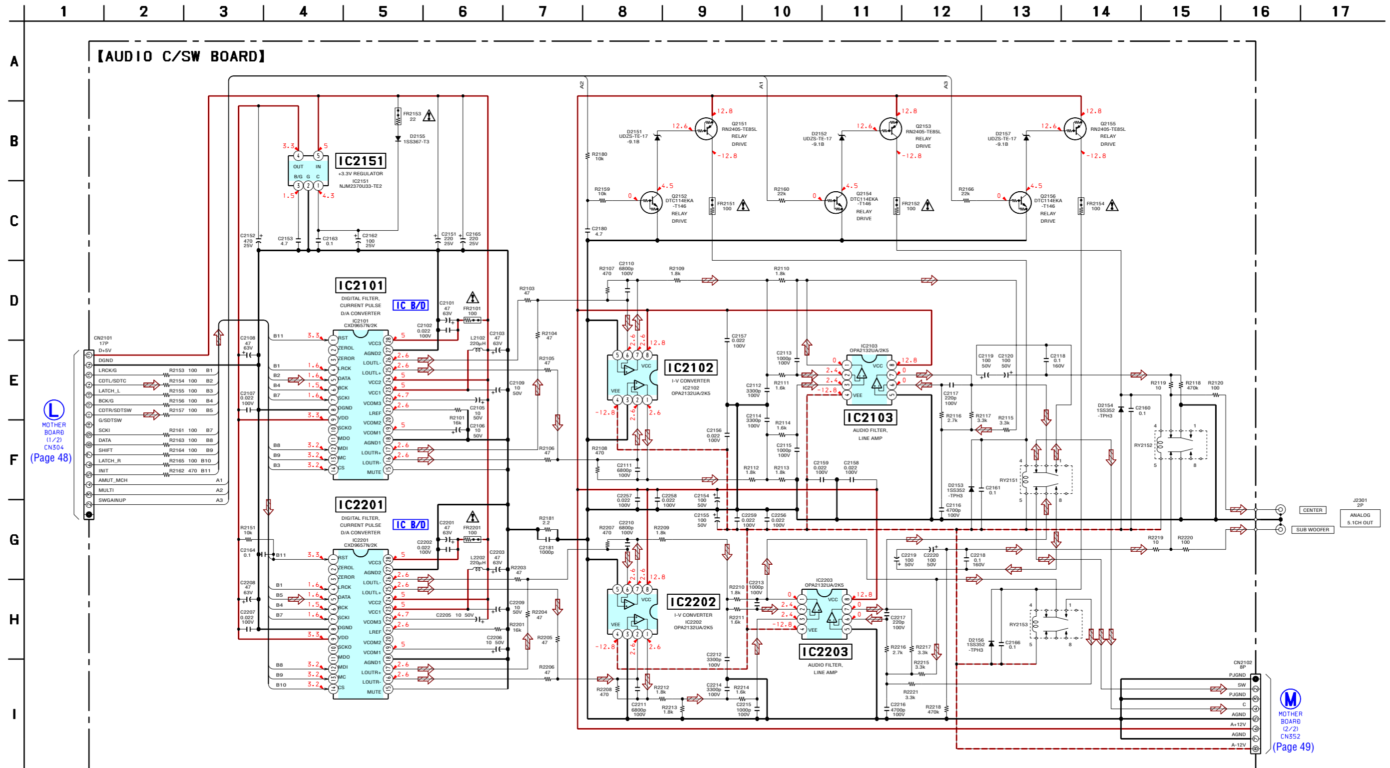
5-31. SCHEMATIC DIAGRAM – AUDIO C/SW Board – • See page 70 for IC Block Diagrams.
