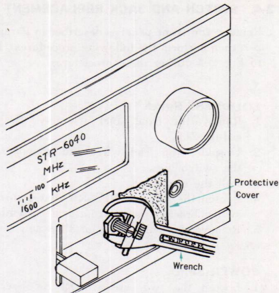
Fig. 2-3 Removal of hexagonal nut
