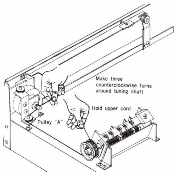
Fig. 2-11 Wrapping dial cord around tuning shaft
