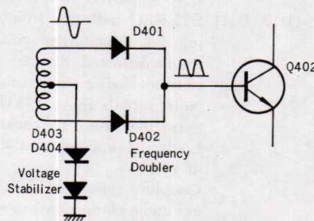
Fig. 1-2 Frequency doubler
