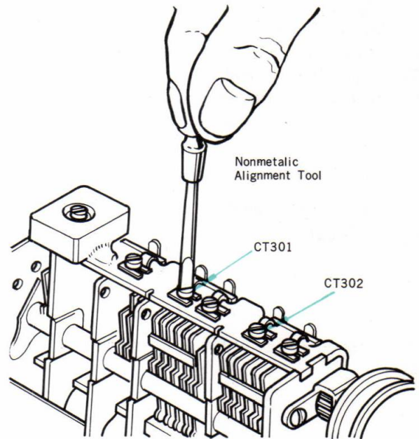
Fig. 3-15 Location of trimmer capacitor CT301 & CT302
