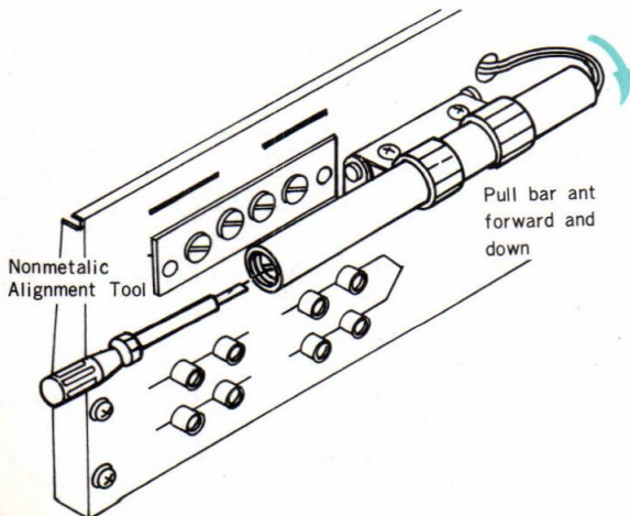
Fig. 3-16 A-m bar antenna core adjustment
