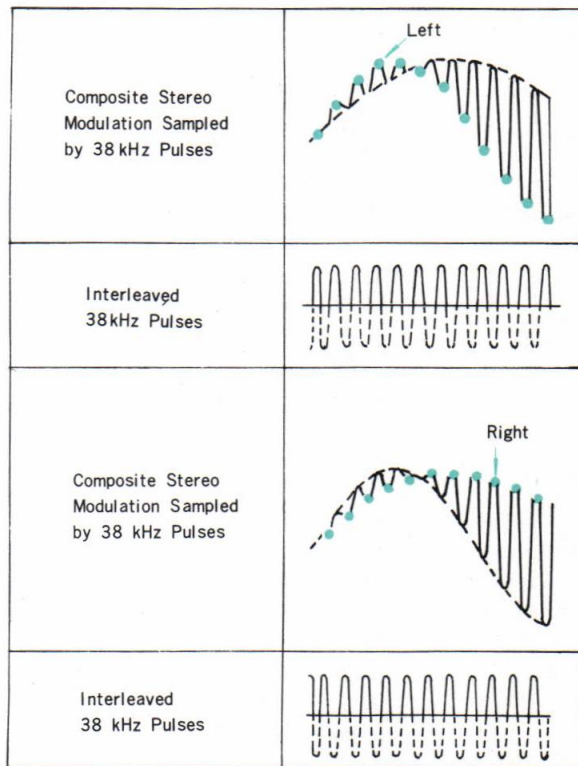
Fig. 1-5 Stereo switching mode
