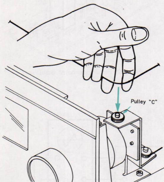
Fig. 2-13 Threading the dial cord over pulley "C"
