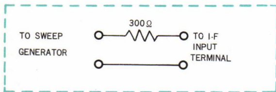
Fig. 3-1 Dummy circuit
