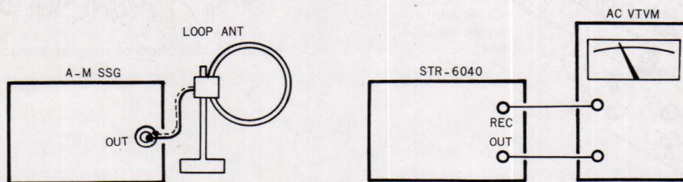
Fig. 3-13 A-m tuner frequency coverage and tracking alignment test set-up
