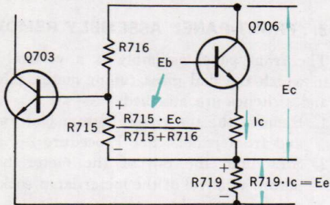
Fig. 1-6 Driver limiter
