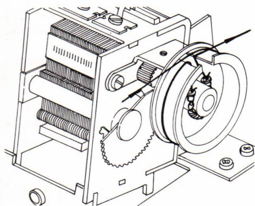
Fig. 2-9 Location of tension spring and dial-cord
