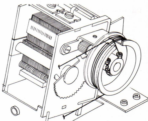
Fig. 2-10 Wrapping dial cord around tuning drum
