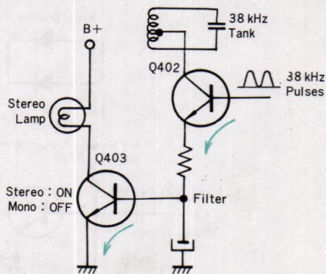
Fig. 1-3 Stereo lamp circuit
