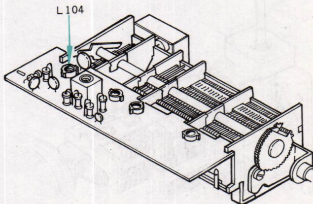
Fig. 3-7 Location of fm oscillator coil L104
