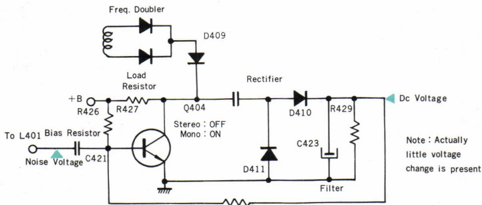
Fig. 1-4 Noise amplifier
