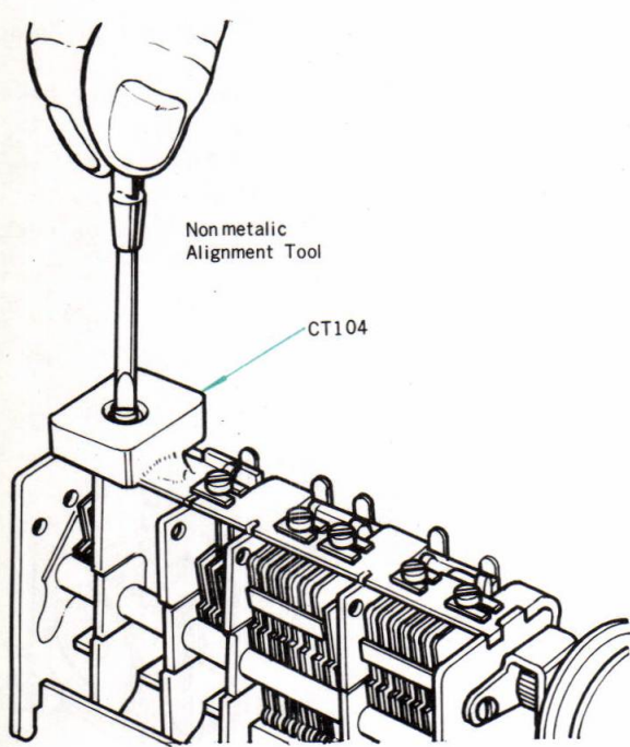
Fig. 3-8 Location of fm trimmer capacitor CT104
