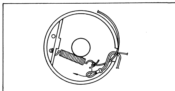
Fig. 2-11 Finishing dial cord stringing
