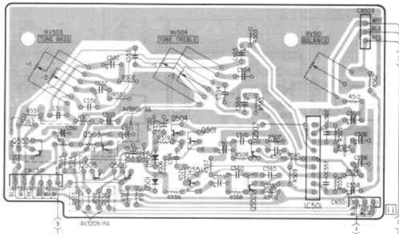
[TONE BOARD]
