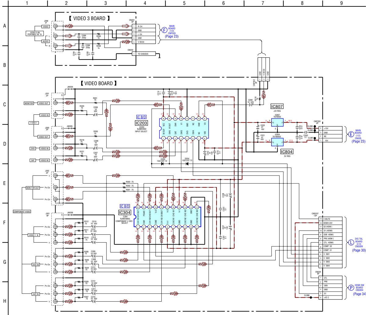
5-17. SCHEMATIC DIAGRAM — VIDEO SECTION — • Refer to page 43 for IC Block Diagrams.
