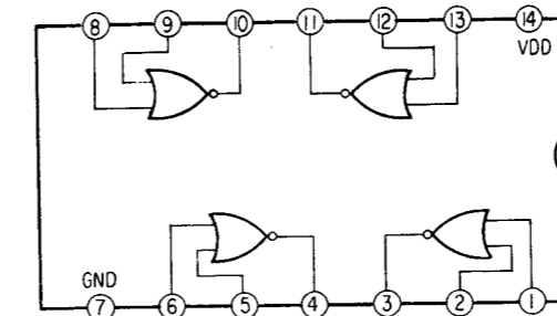
IC705 MB84001B
