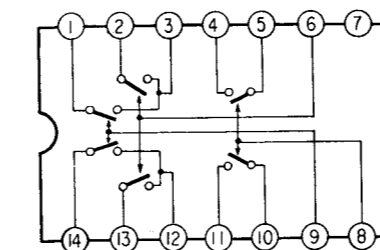
IC803 CX770
