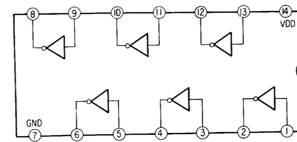
IC704 MB84069B
