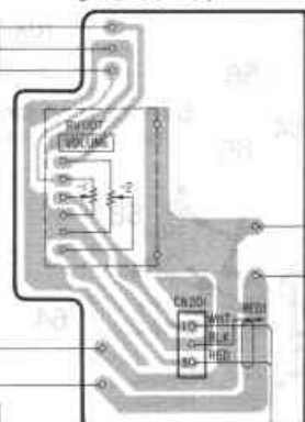
[VOL BOARD]
