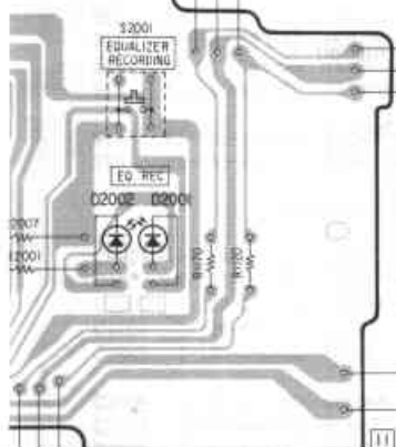
[VOL BOARD]
