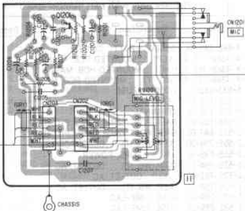
[MICROPHONE BOARD]
