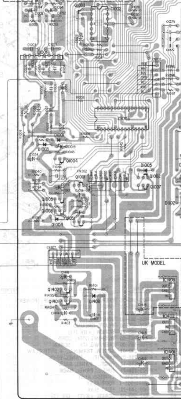
[MOTOR BOARD]
