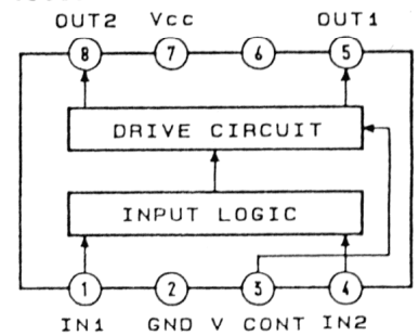
IC803 LB1639
