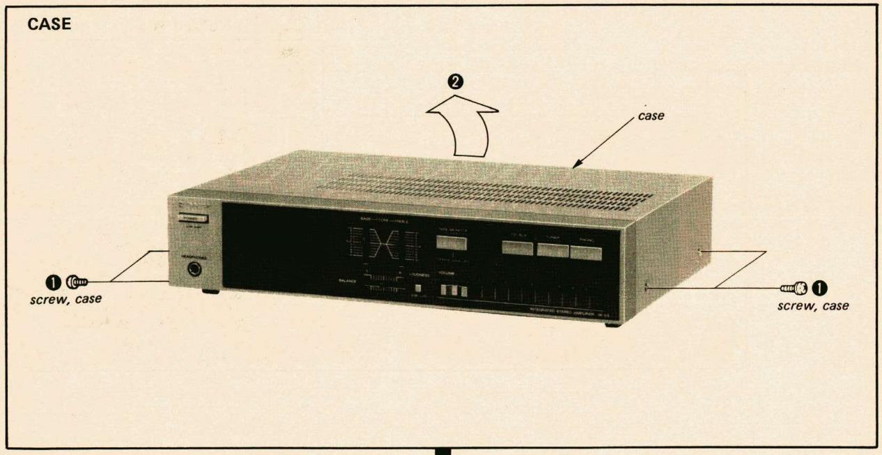
2-1. REMOVAL
