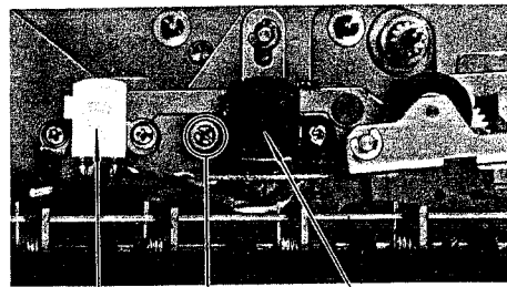
erase head record/playback head adjustment screw
