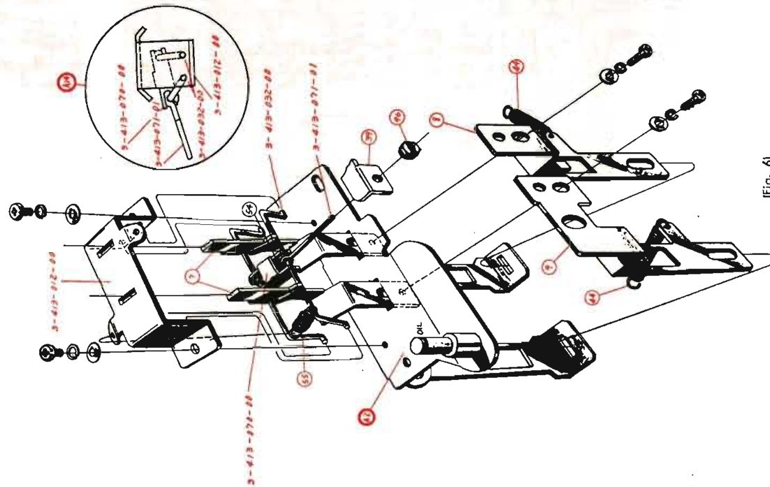
Record Button Mechanism—Top View
