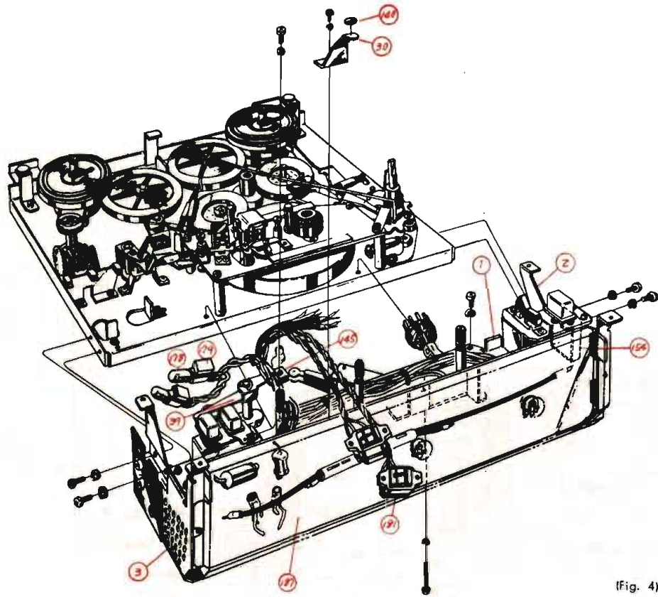
Chassis—Top View
