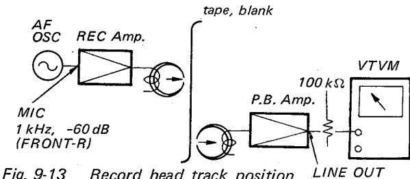
Fig. 9-13 Record head track position adjustment setup
