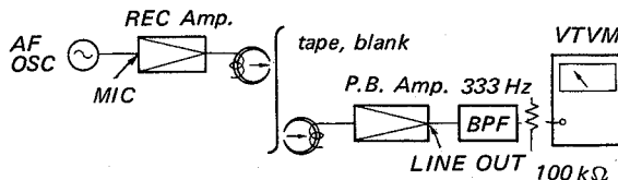
Fig. 9-21 Erase ratio measurement setup
