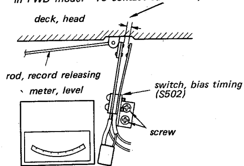
Fig. 8-15 Bias timing switch position adjustment
