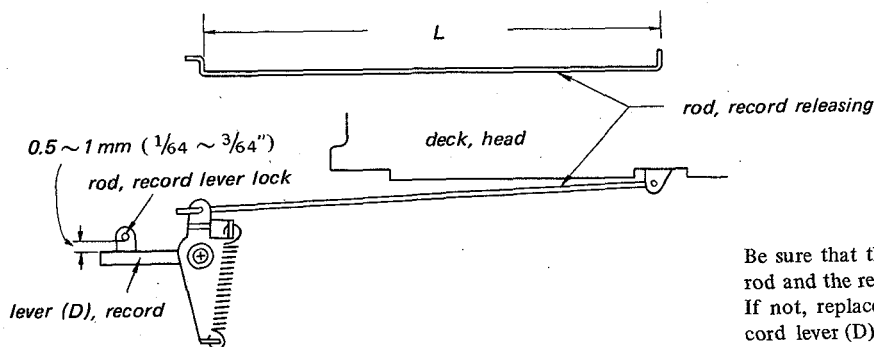
Fig. 8-27 Record releasing rod adjustment
