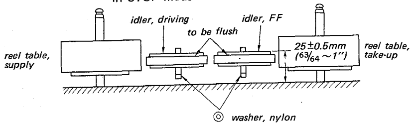
Fig. 8-26 FF & Driving idler height adjustments
