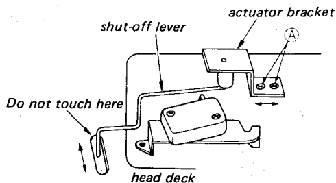
Fig. 5-1-1. Automatic shut-off switch adjustment (1)
