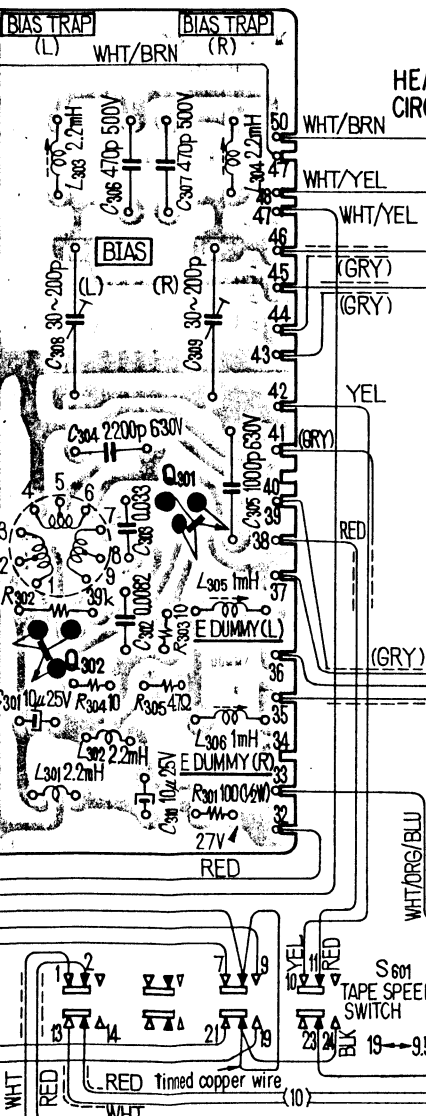
RD AMP and BIAS OSC CIRCUIT BOARD
