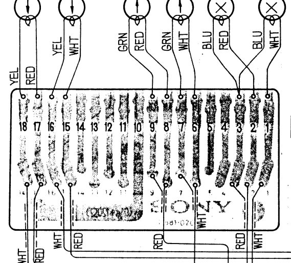
PLAY PF140-4202 H606 (R) H605 (L) REC RF140-2902 H604 (R) H603 (L) E EF 12 -2902A2 H602 (R) H601 (L)
