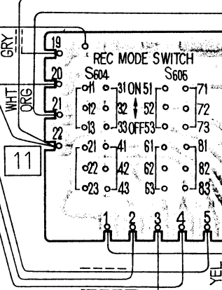
REC MODE CIRCUIT BOARD
