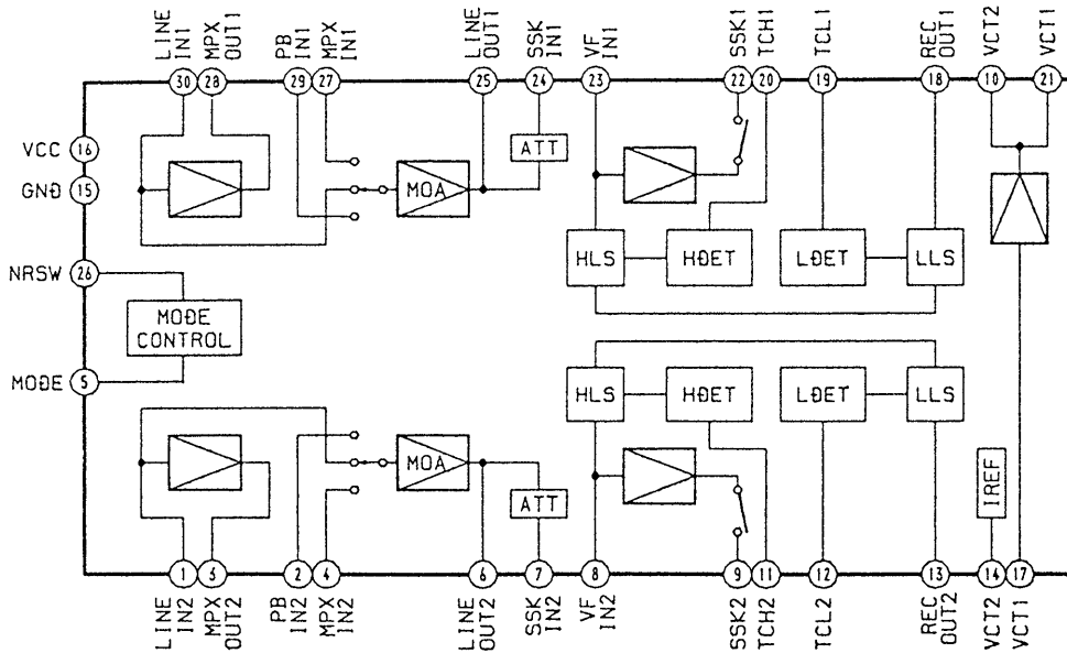
IC103 CXA1331S
