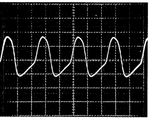
4 IC601 ㉓pin (X OUT), IC602 ⑳pin (X IN) 5.6Vp-p, 0.25μsec
