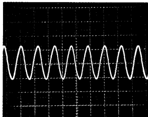
8 IC351 ④⑤pin (OSC1) 4.8Vp-p, 0.24μsec
