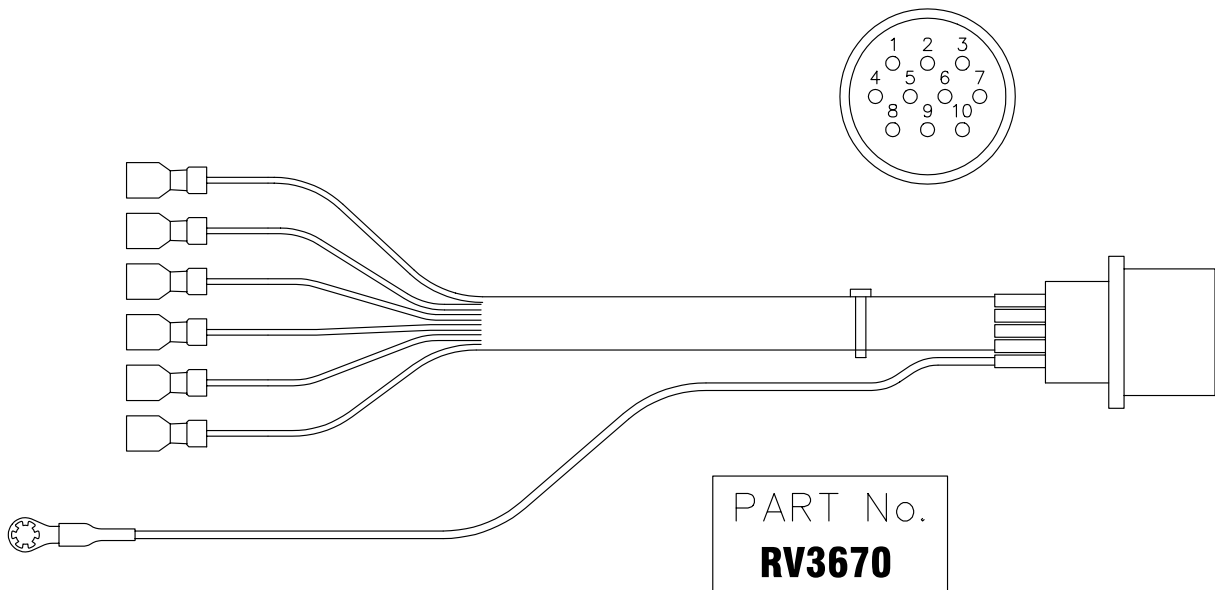
REAR VIEW OF SRC (VIEWED FROM INSIDE PSU)
